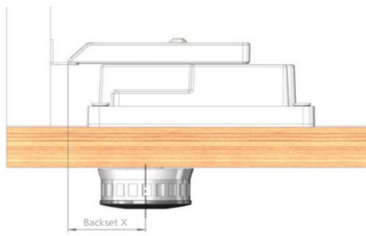
Adjustable Backset 33.5 mm – 56.2 mm
