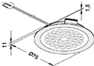
Foco redondo R68
